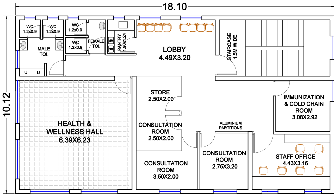
FIRST FLOOR PLAN (BUILTUP AREA = 183.22 SQ.M.)
