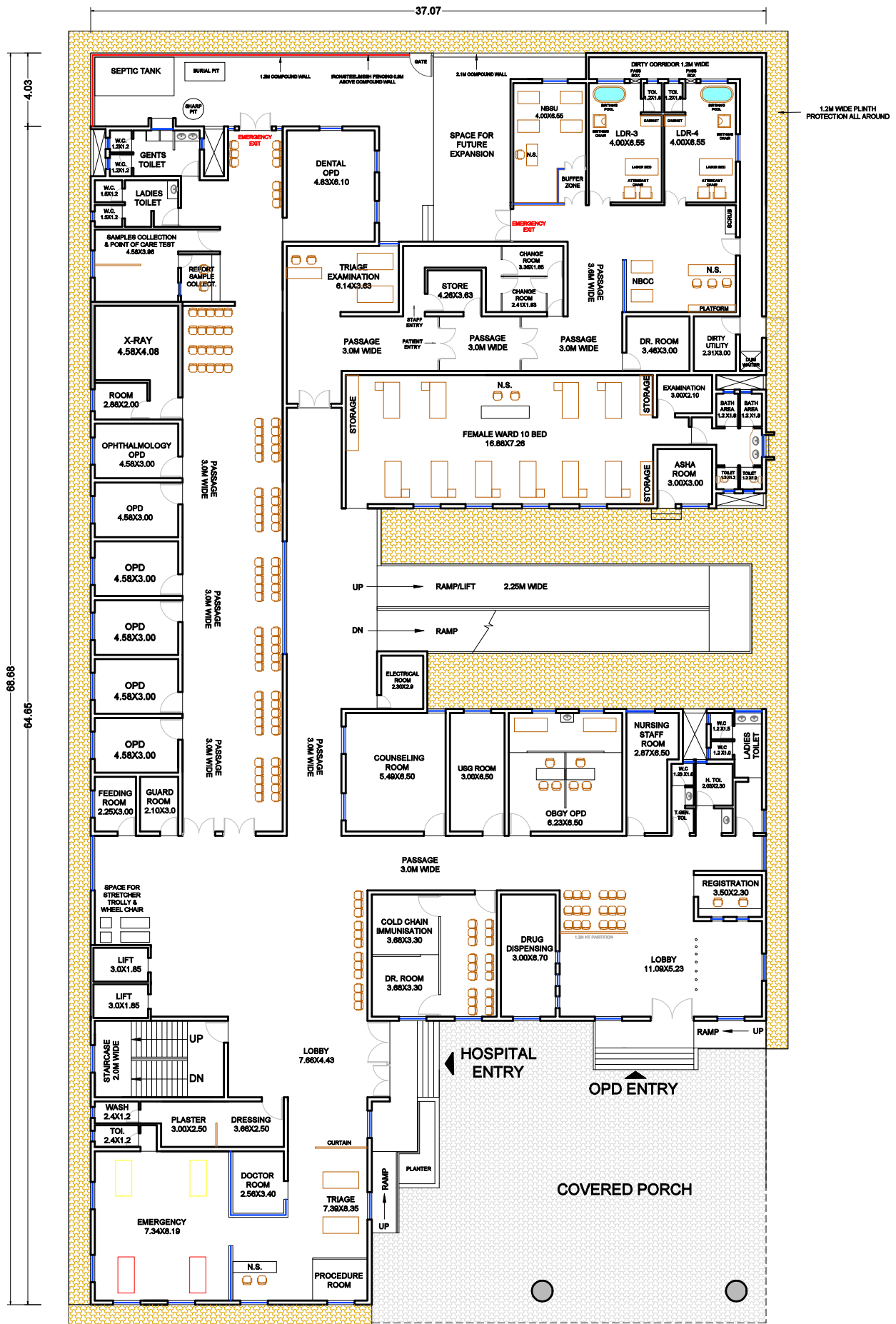
GROUND FLOOR PLAN AREA 1928.00 SQ.M
