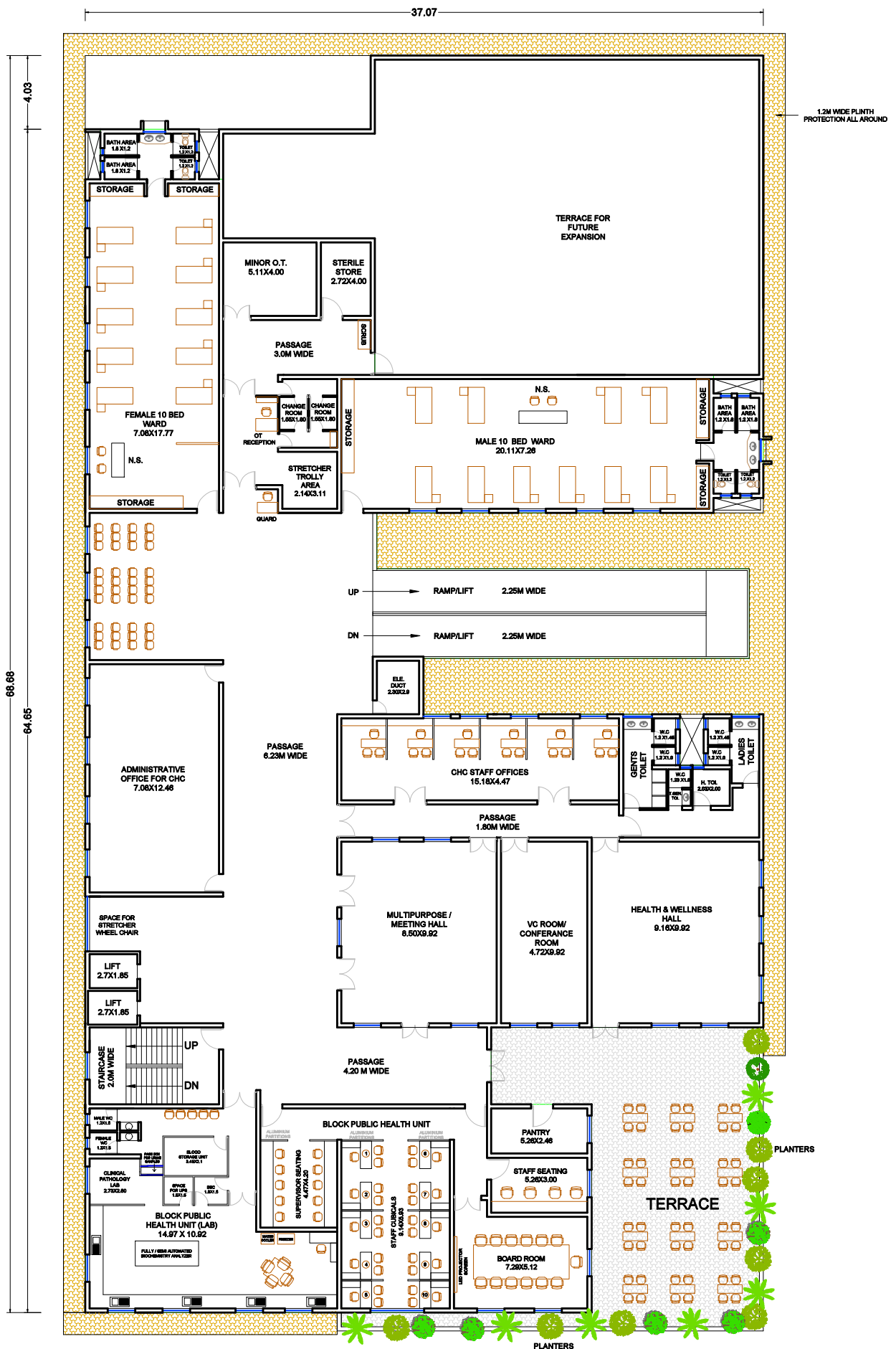
FIRST FLOOR PLAN AREA 1753.00 SQ.M
