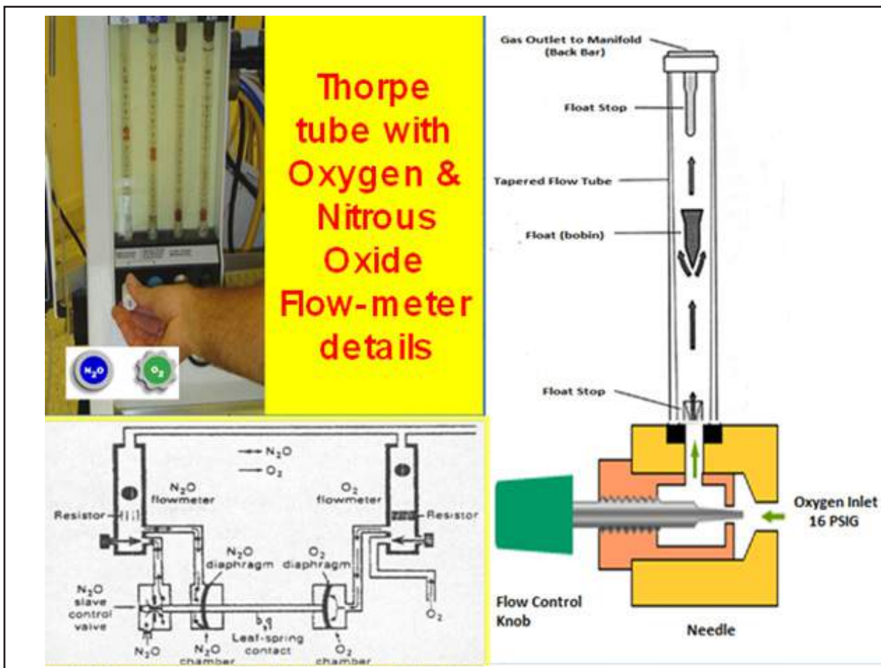
Figure 9: Flowmeter
