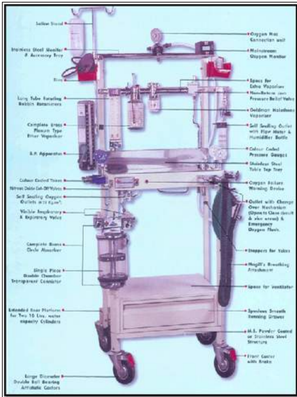
Figure10: Boyle's machine
